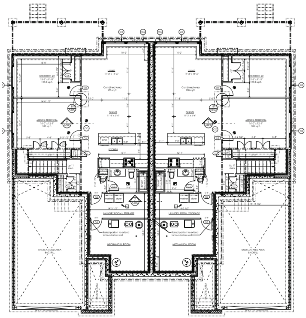
BASEMENT PLAN SCALE: 1/8" = 1'-0"
